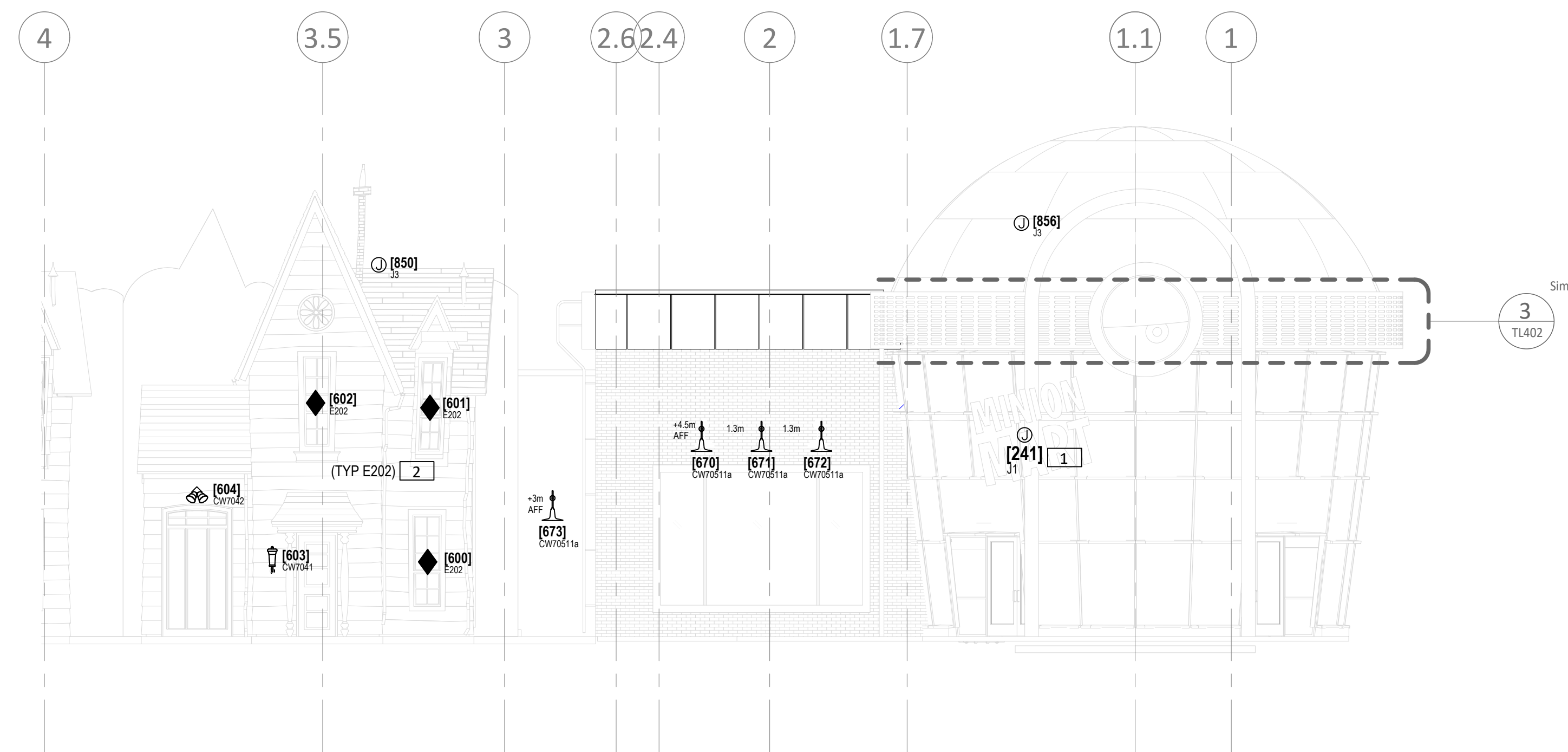
2 ELEVATION - NORTH - THEMED LIGHTING TL201
